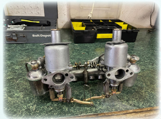
Restored carburetors by Bob Abbott of British Car R&R.
