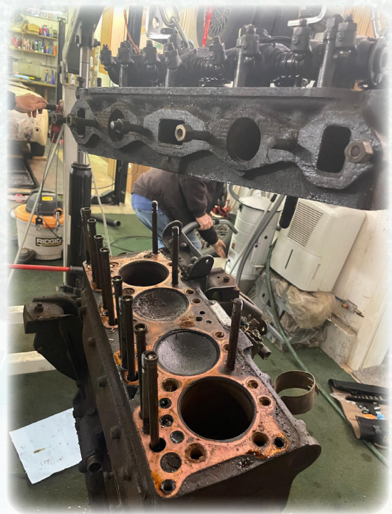
Head removed from 100 Block
