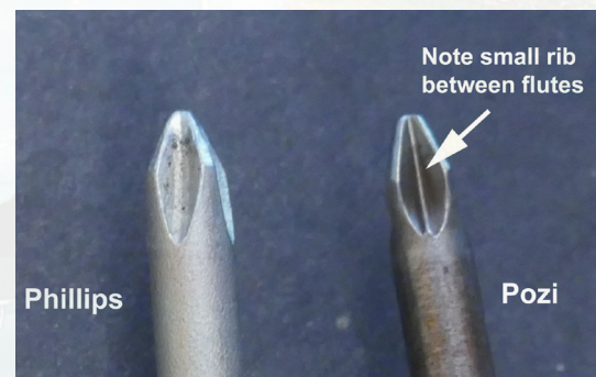
This photo shows how the appearance differs between the tips of Phillips (left) and Pozi (right) screwdrivers.
